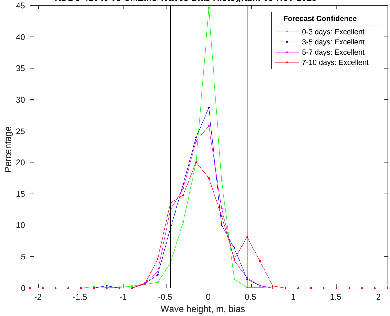
NDBC 41040 vs CMEMS Waves Bias Histogram: 05-Nov-2025
