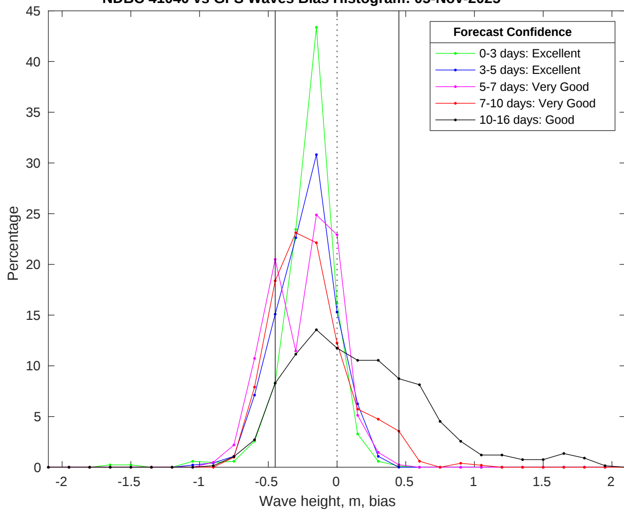
NDBC 41040 vs GFS Waves Bias Histogram: 05-Nov-2025
