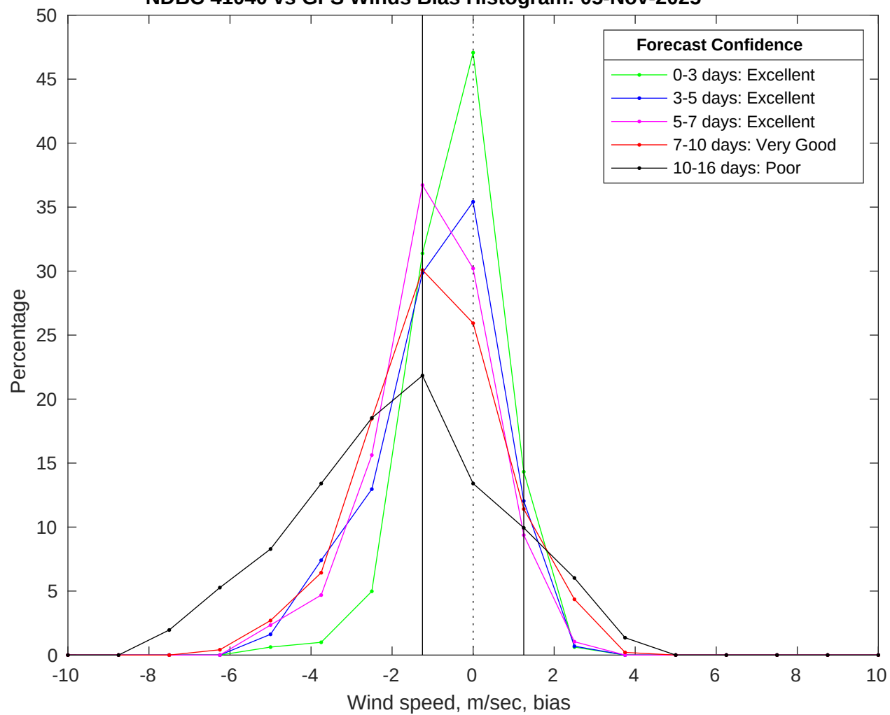
NDBC 41040 vs GFS Winds Bias Histogram: 05-Nov-2025
