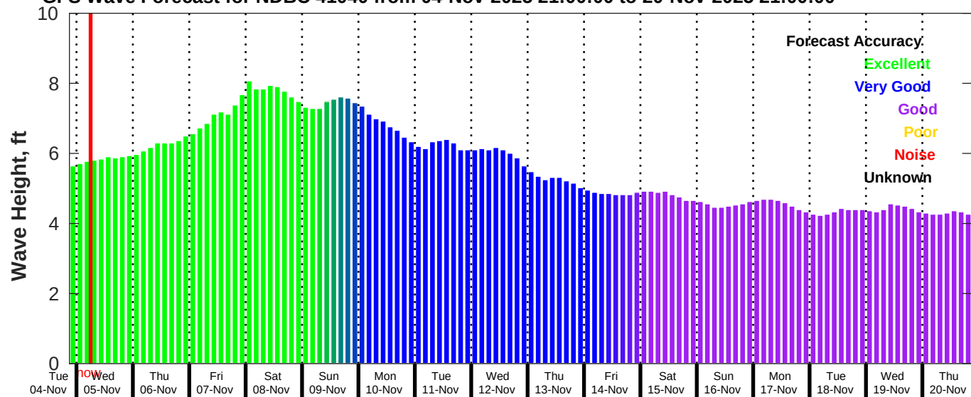
GFS Wave Forecast for NDBC 41040 from 04-Nov-2025 21:00:00 to 20-Nov-2025 21:00:00
