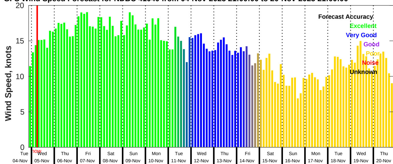
GFS Wind Speed Forecast for NDBC 41040 from 04-Nov-2025 21:00:00 to 20-Nov-2025 21:00:00
