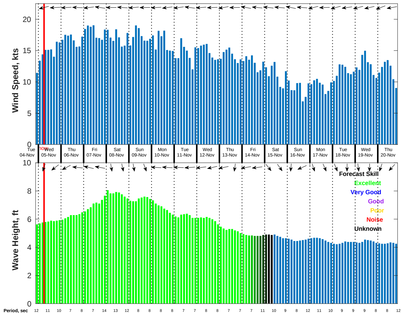
Wind & Wave Forecast for NDBC 41040 from 04-Nov-2025 21:00:00 to 20-Nov-2025 21:00:00
