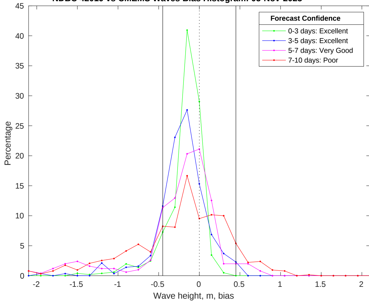
NDBC 42019 vs CMEMS Waves Bias Histogram: 05-Nov-2025
