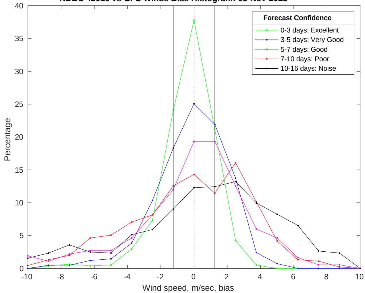
NDBC 42019 vs GFS Winds Bias Histogram: 05-Nov-2025
