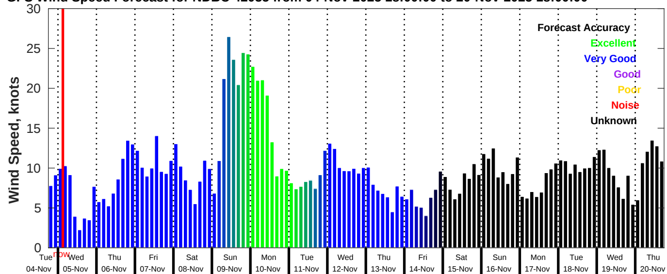
GFS Wind Speed Forecast for NDBC 42035 from 04-Nov-2025 18:00:00 to 20-Nov-2025 18:00:00
