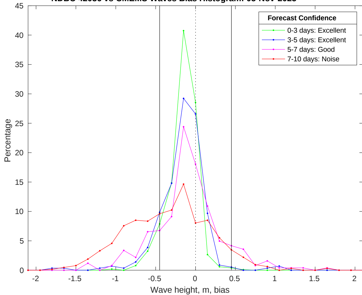
NDBC 42036 vs CMEMS Waves Bias Histogram: 05-Nov-2025
