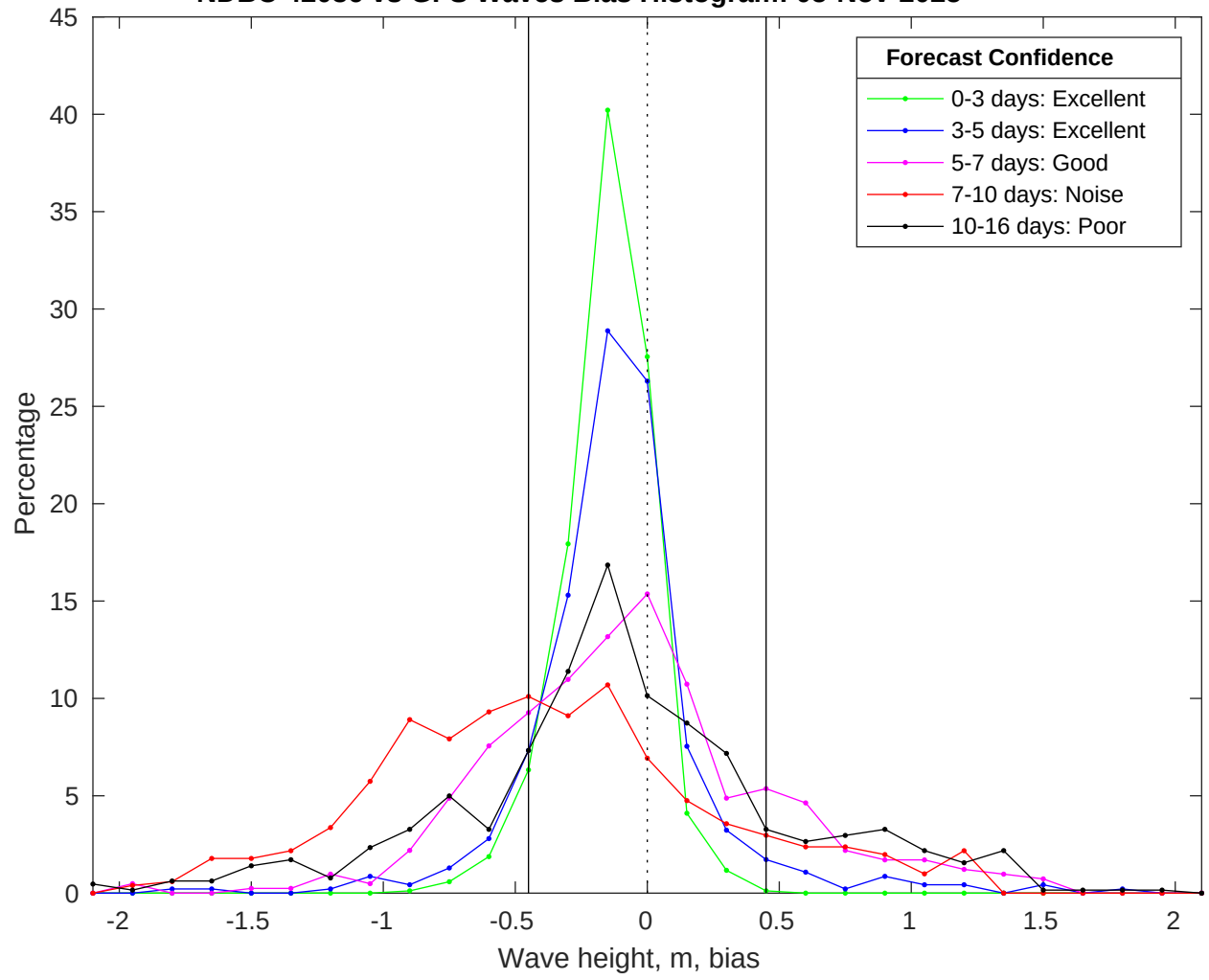
NDBC 42036 vs GFS Waves Bias Histogram: 05-Nov-2025
