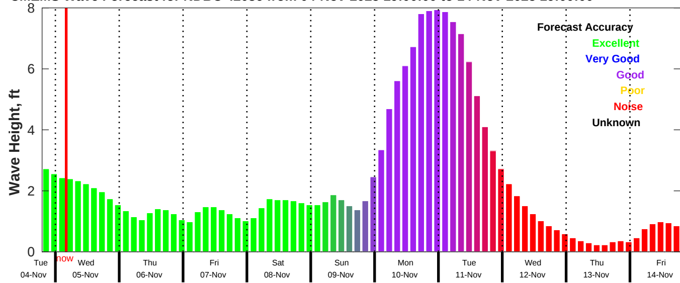
CMEMS Wave Forecast for NDBC 42036 from 04-Nov-2025 19:00:00 to 14-Nov-2025 19:00:00
