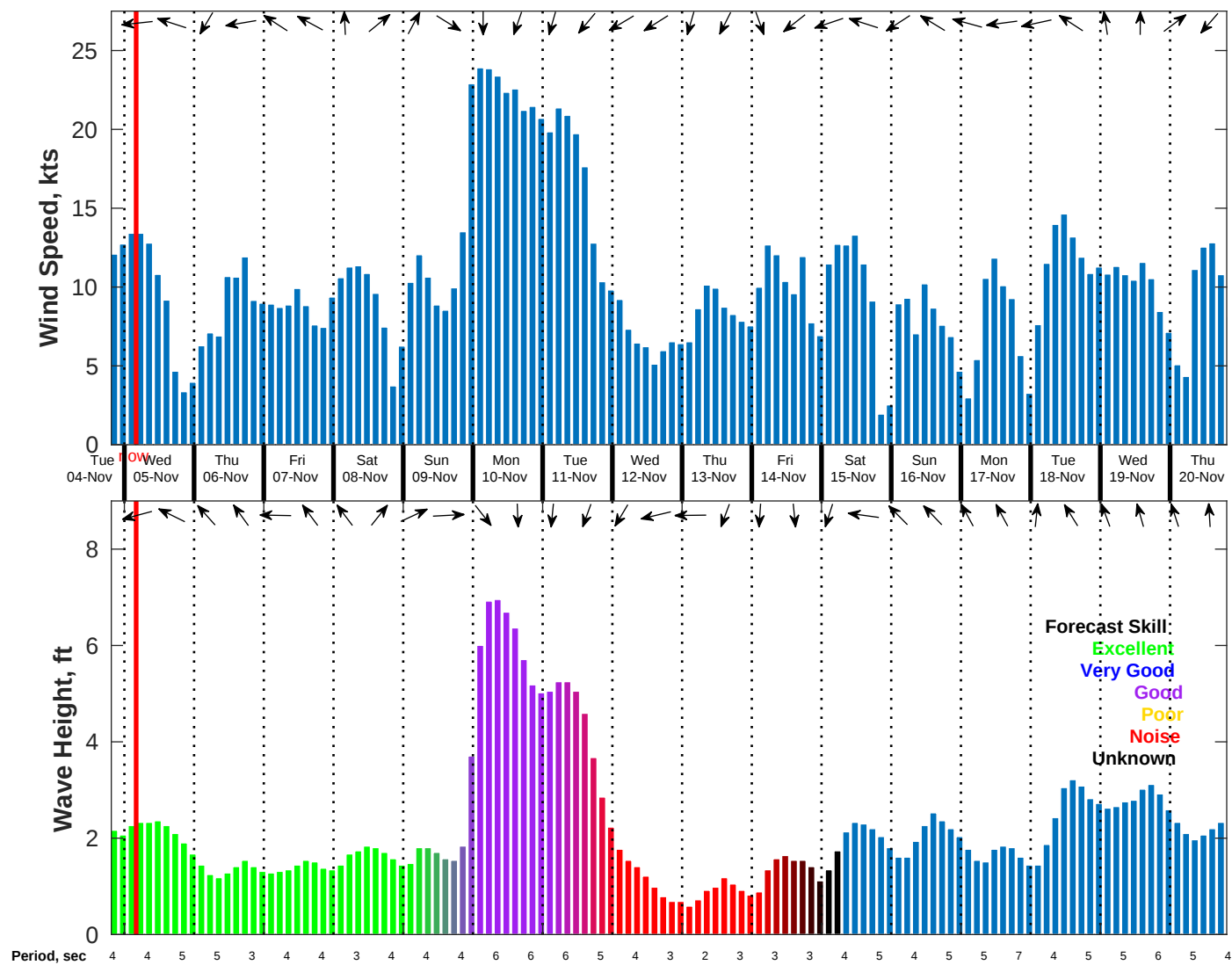
Wind & Wave Forecast for NDBC 42036 from 04-Nov-2025 19:00:00 to 20-Nov-2025 19:00:00
