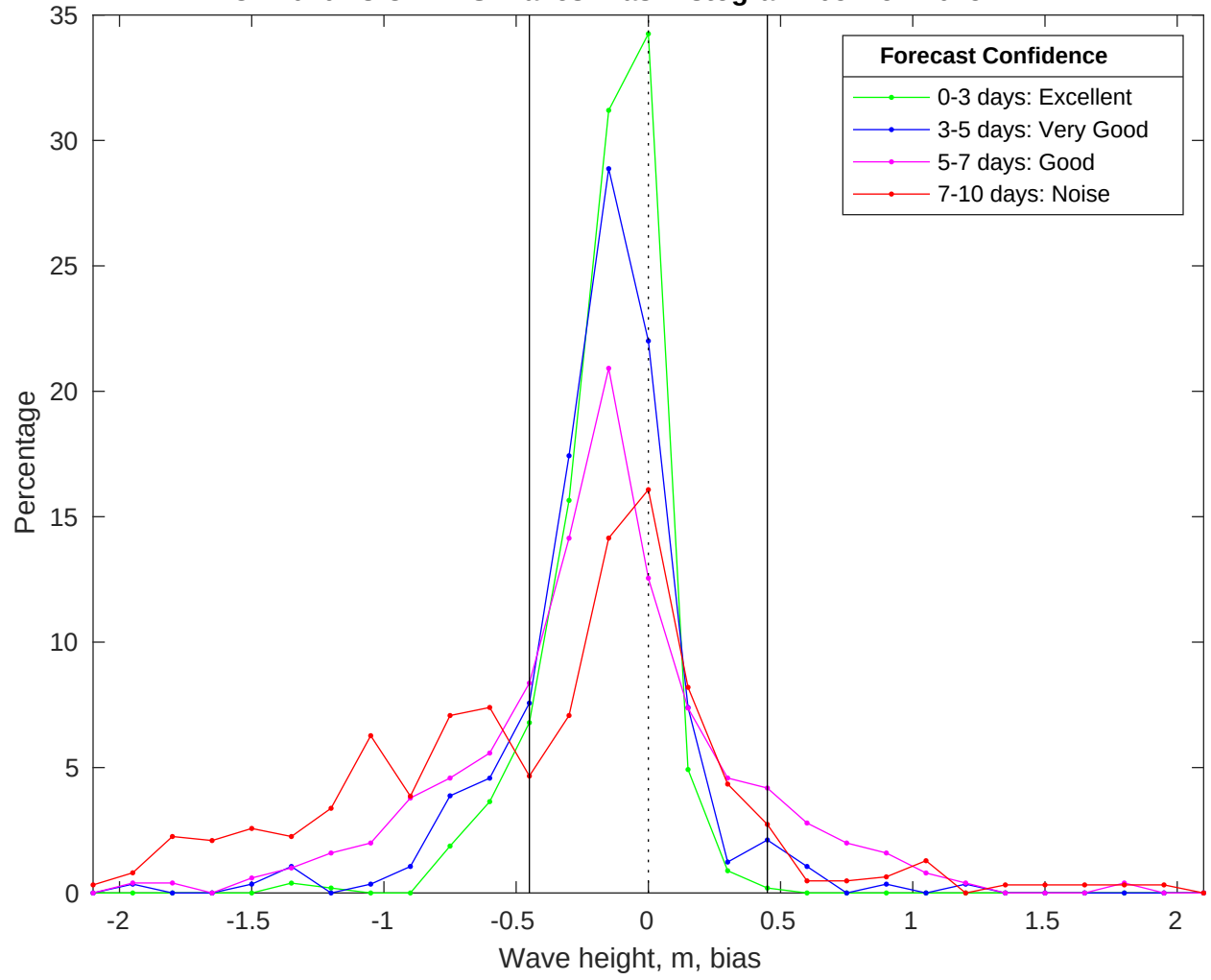
NDBC 42040 vs CMEMS Waves Bias Histogram: 05-Nov-2025
