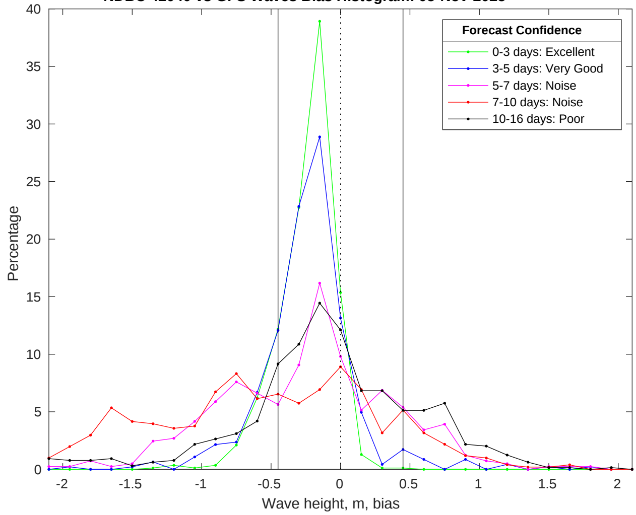
NDBC 42040 vs GFS Waves Bias Histogram: 05-Nov-2025
