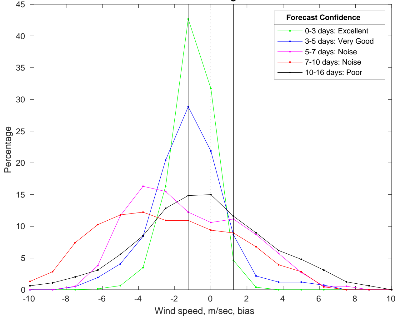
NDBC 42040 vs GFS Winds Bias Histogram: 05-Nov-2025
