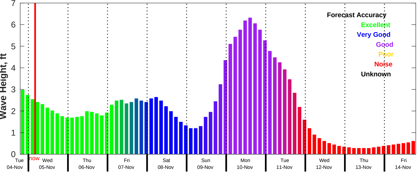
CMEMS Wave Forecast for NDBC 42040 from 04-Nov-2025 19:00:00 to 14-Nov-2025 19:00:00
