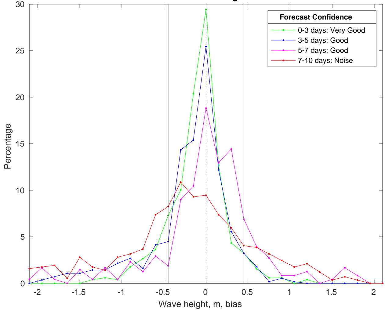
NDBC 44008 vs CMEMS Waves Bias Histogram: 05-Nov-2025
