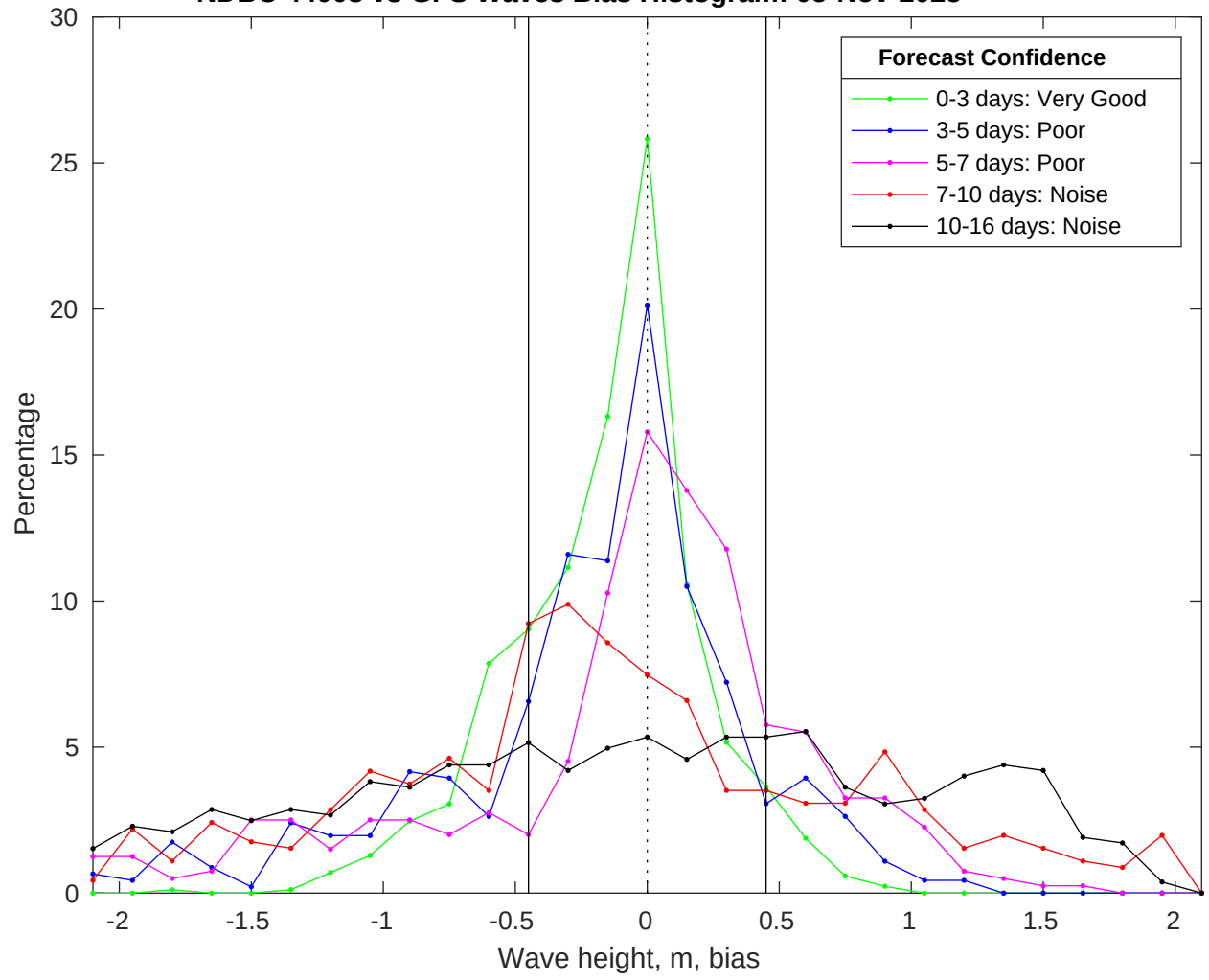
NDBC 44008 vs GFS Waves Bias Histogram: 05-Nov-2025
