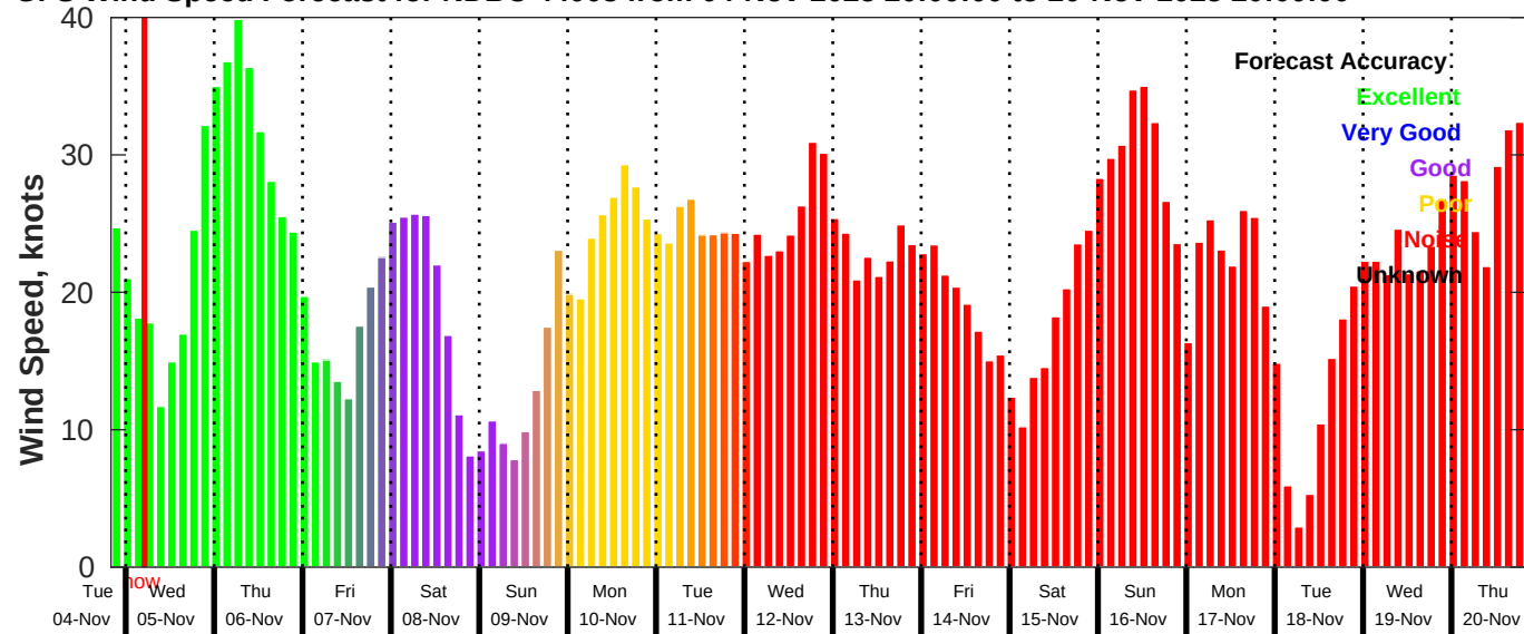
GFS Wind Speed Forecast for NDBC 44008 from 04-Nov-2025 20:00:00 to 20-Nov-2025 20:00:00
