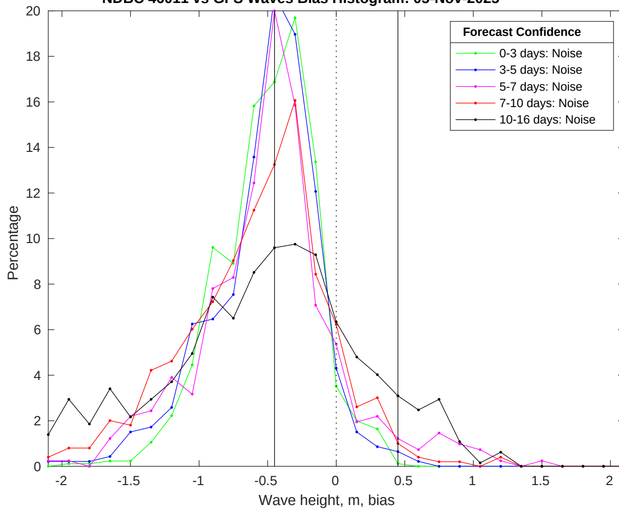
NDBC 46011 vs GFS Waves Bias Histogram: 05-Nov-2025
