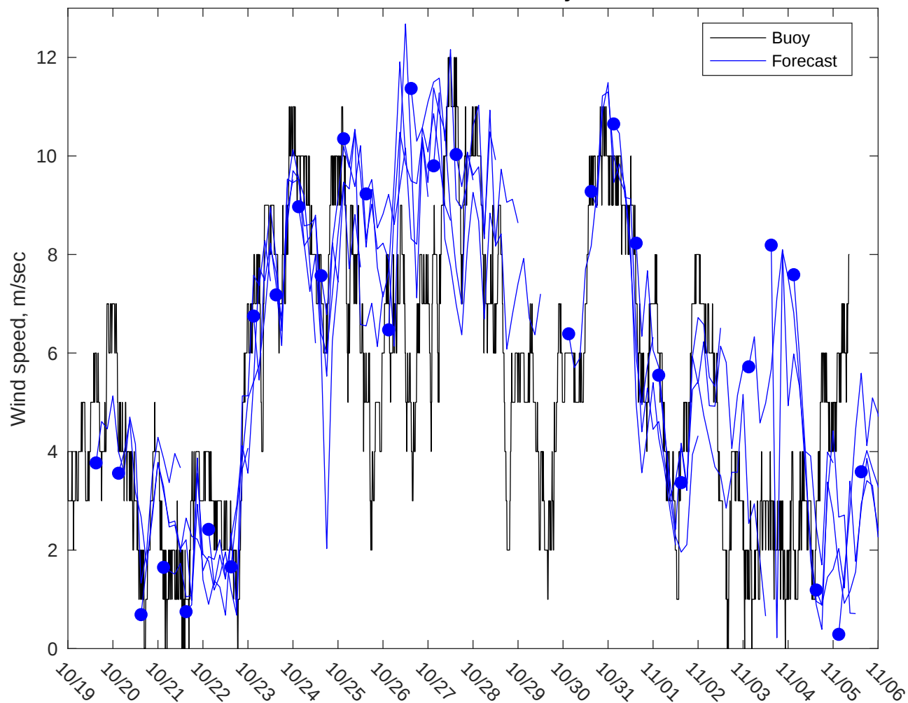
NDBC 46011 vs GFS Winds: 3 to 5 day forecast
