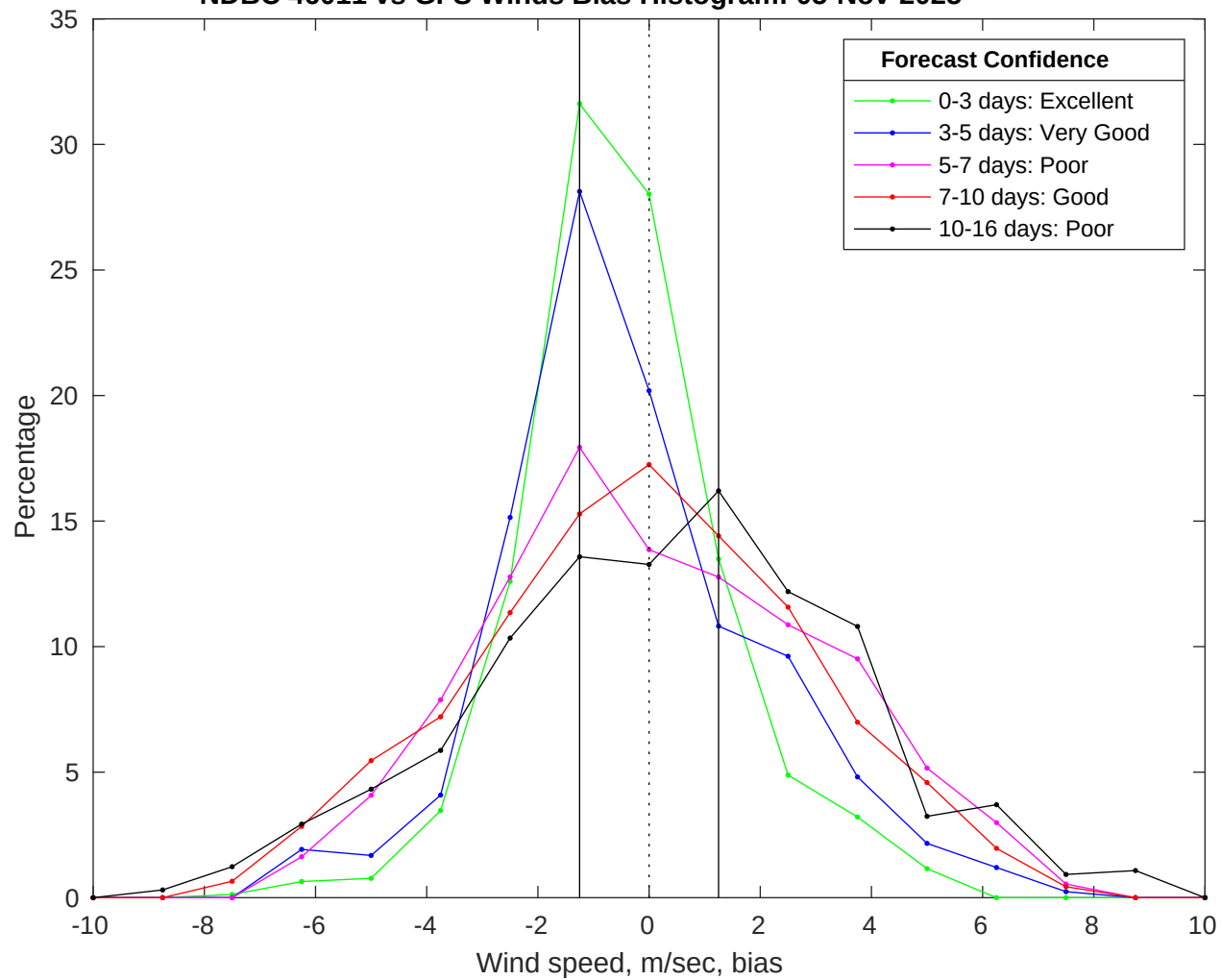
NDBC 46011 vs GFS Winds Bias Histogram: 05-Nov-2025
