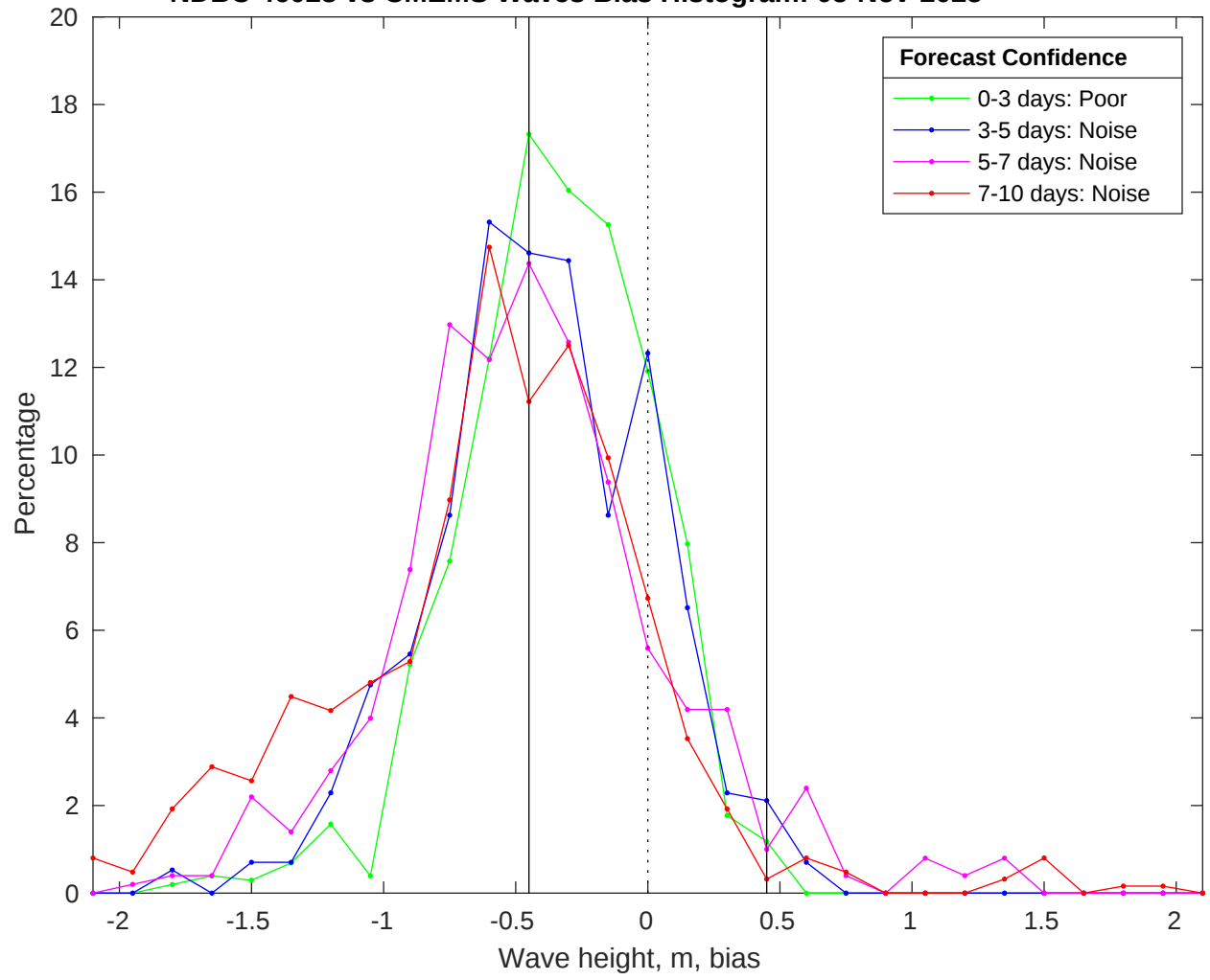
NDBC 46028 vs CMEMS Waves Bias Histogram: 05-Nov-2025
