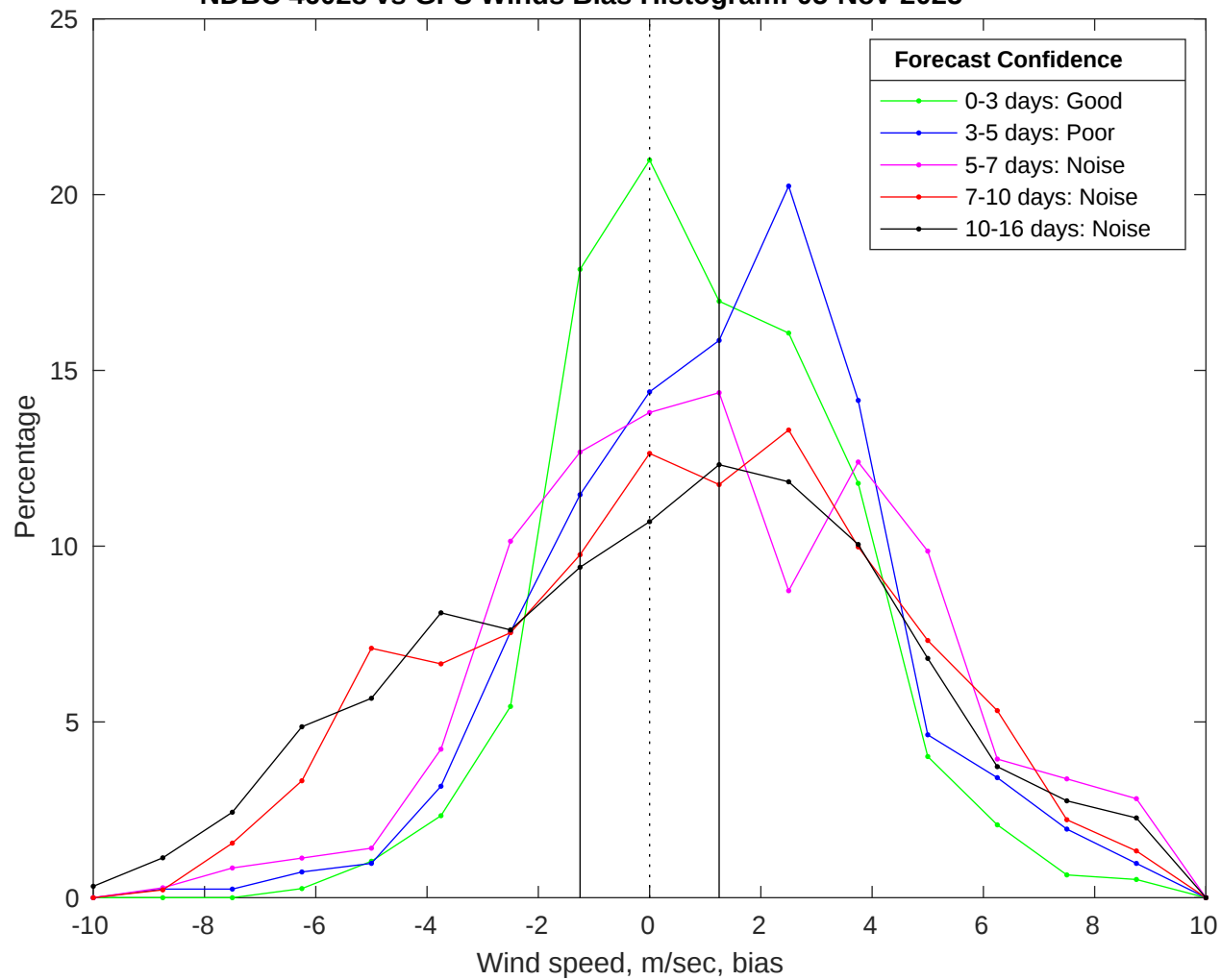
NDBC 46028 vs GFS Winds Bias Histogram: 05-Nov-2025
