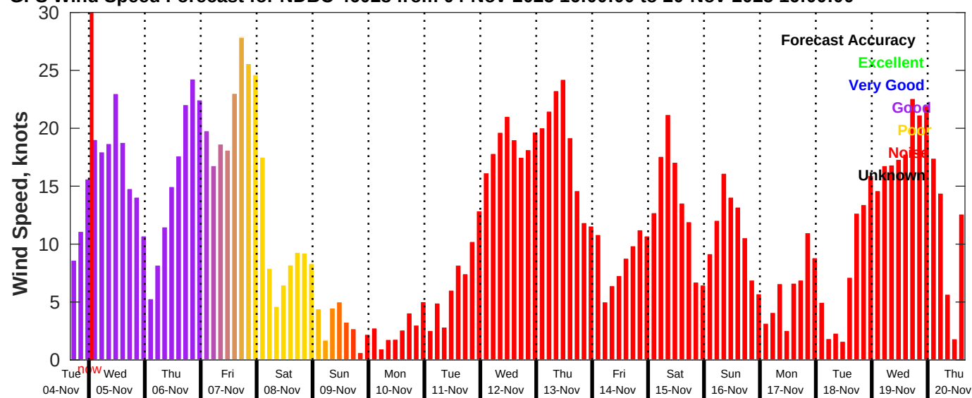
GFS Wind Speed Forecast for NDBC 46028 from 04-Nov-2025 16:00:00 to 20-Nov-2025 16:00:00
