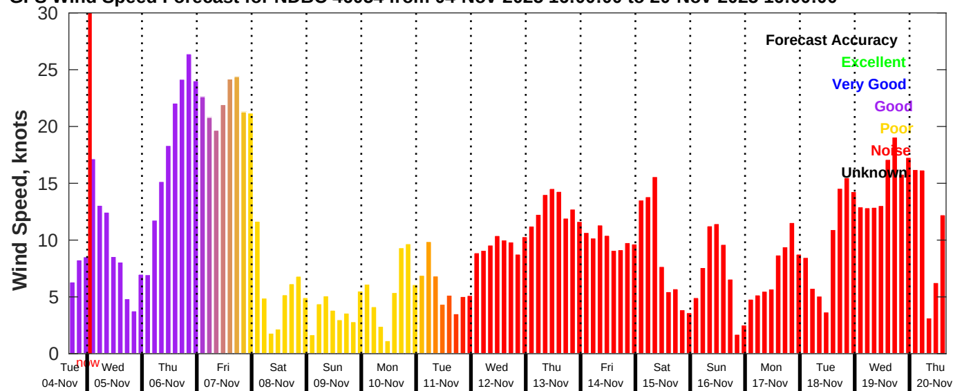
GFS Wind Speed Forecast for NDBC 46054 from 04-Nov-2025 16:00:00 to 20-Nov-2025 16:00:00
