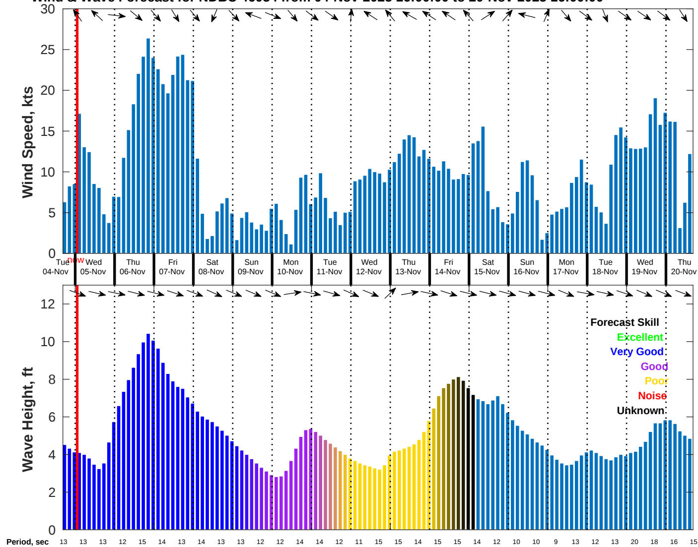
Wind & Wave Forecast for NDBC 46054 from 04-Nov-2025 16:00:00 to 20-Nov-2025 16:00:00
