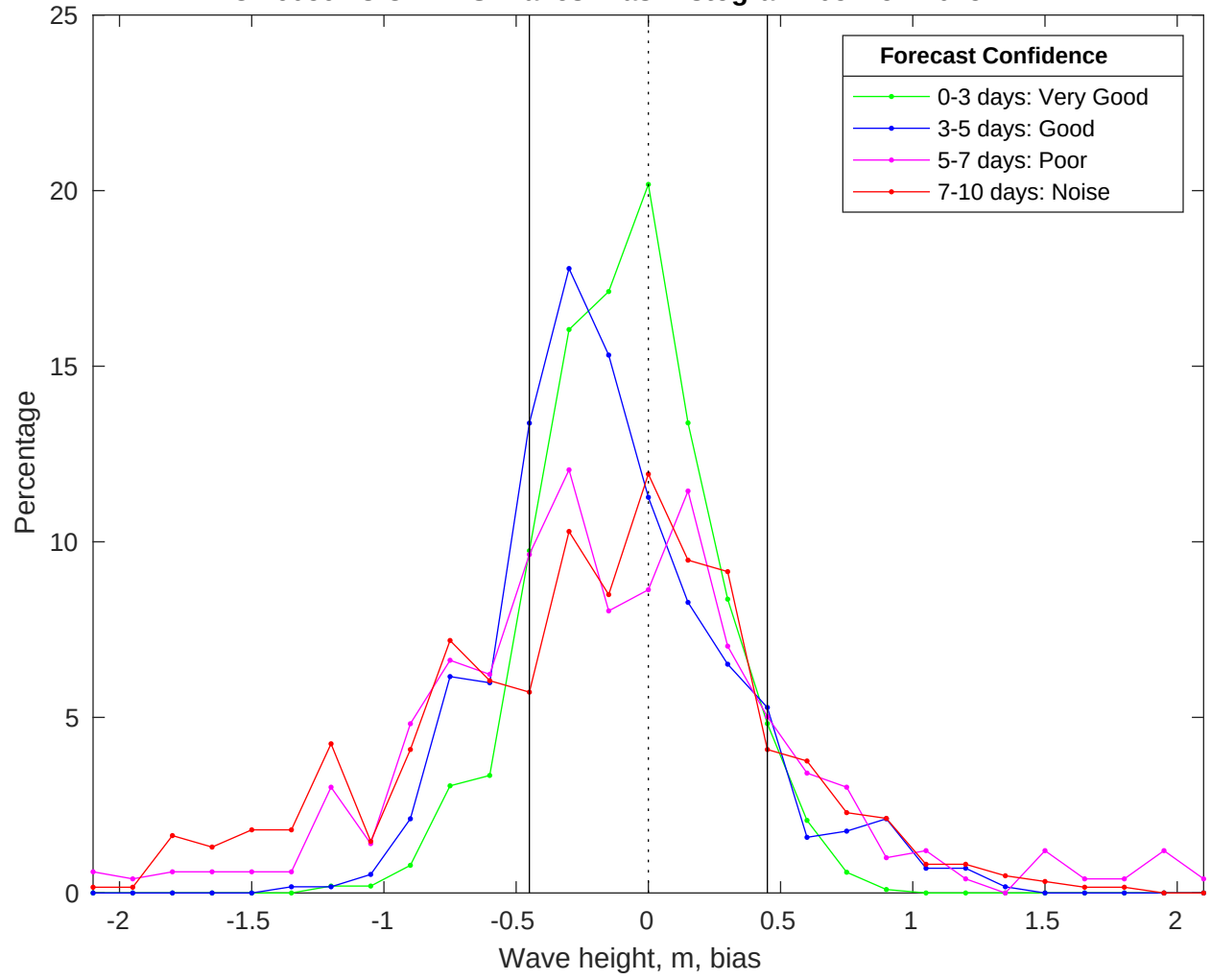
NDBC 46059 vs CMEMS Waves Bias Histogram: 05-Nov-2025
