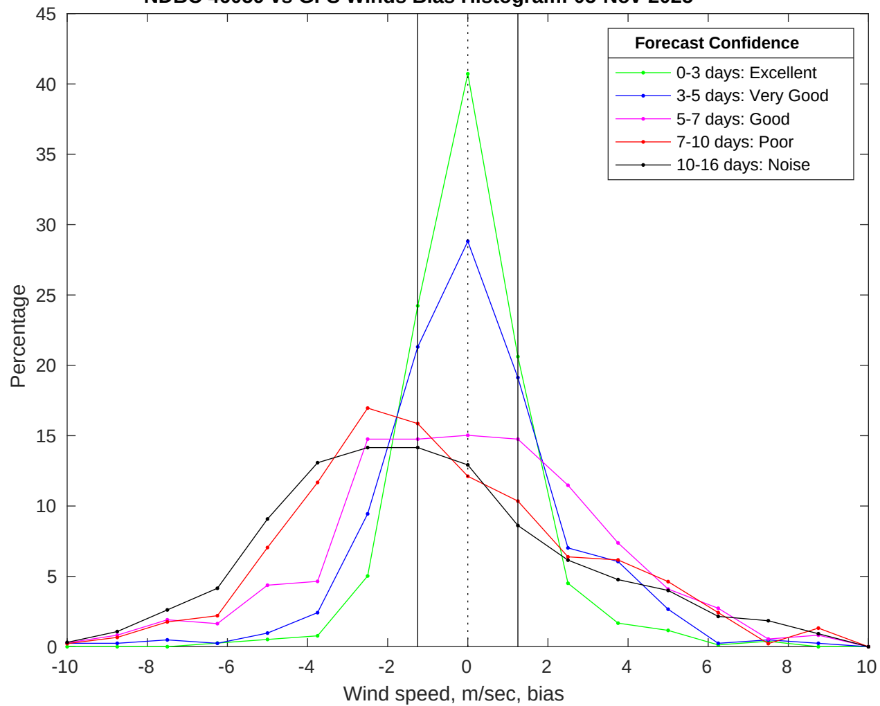
NDBC 46059 vs GFS Winds Bias Histogram: 05-Nov-2025
