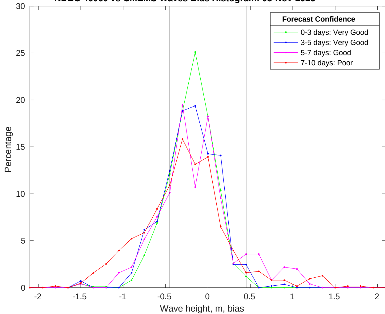
NDBC 46069 vs CMEMS Waves Bias Histogram: 05-Nov-2025
