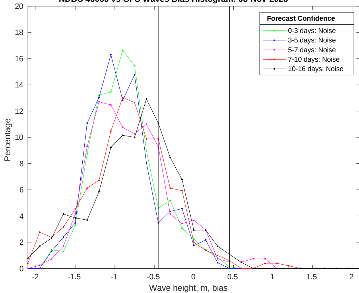
NDBC 46069 vs GFS Waves Bias Histogram: 05-Nov-2025
