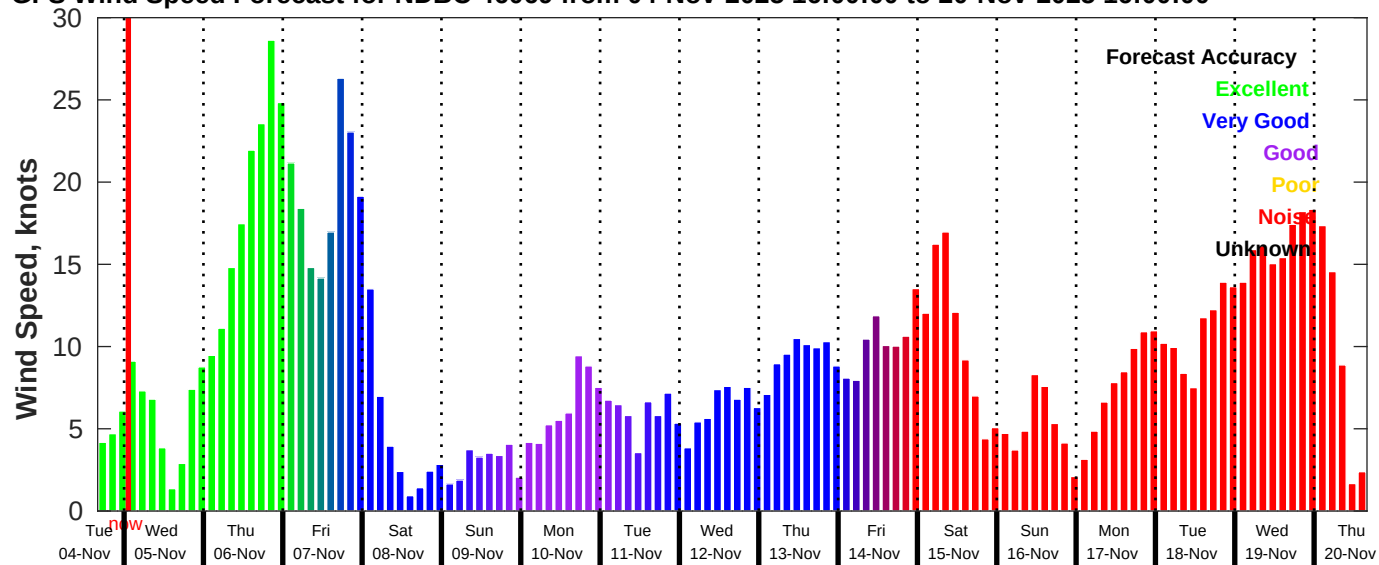
GFS Wind Speed Forecast for NDBC 46069 from 04-Nov-2025 16:00:00 to 20-Nov-2025 16:00:00
