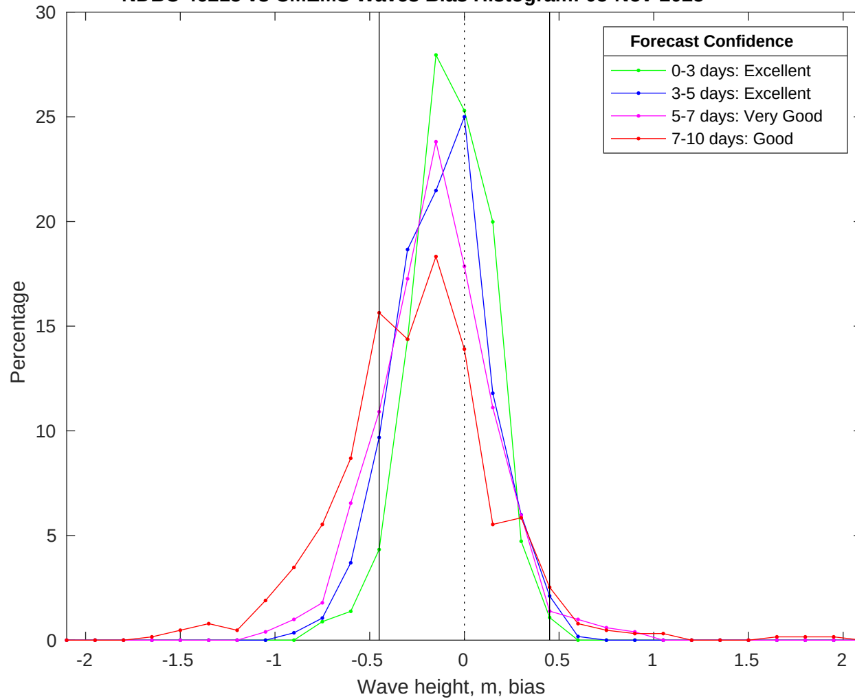
NDBC 46215 vs CMEMS Waves Bias Histogram: 05-Nov-2025
