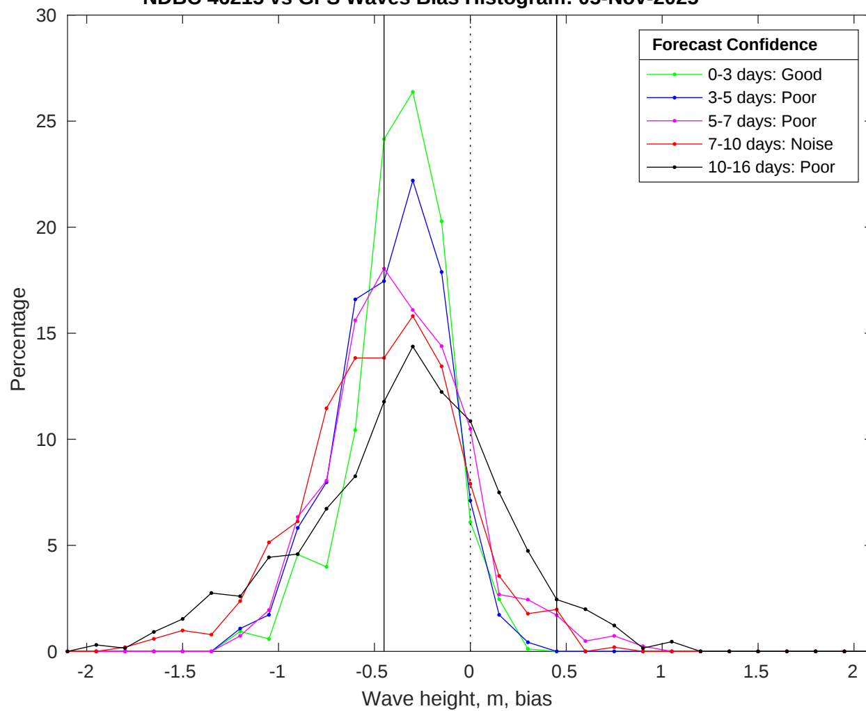
NDBC 46215 vs GFS Waves Bias Histogram: 05-Nov-2025
