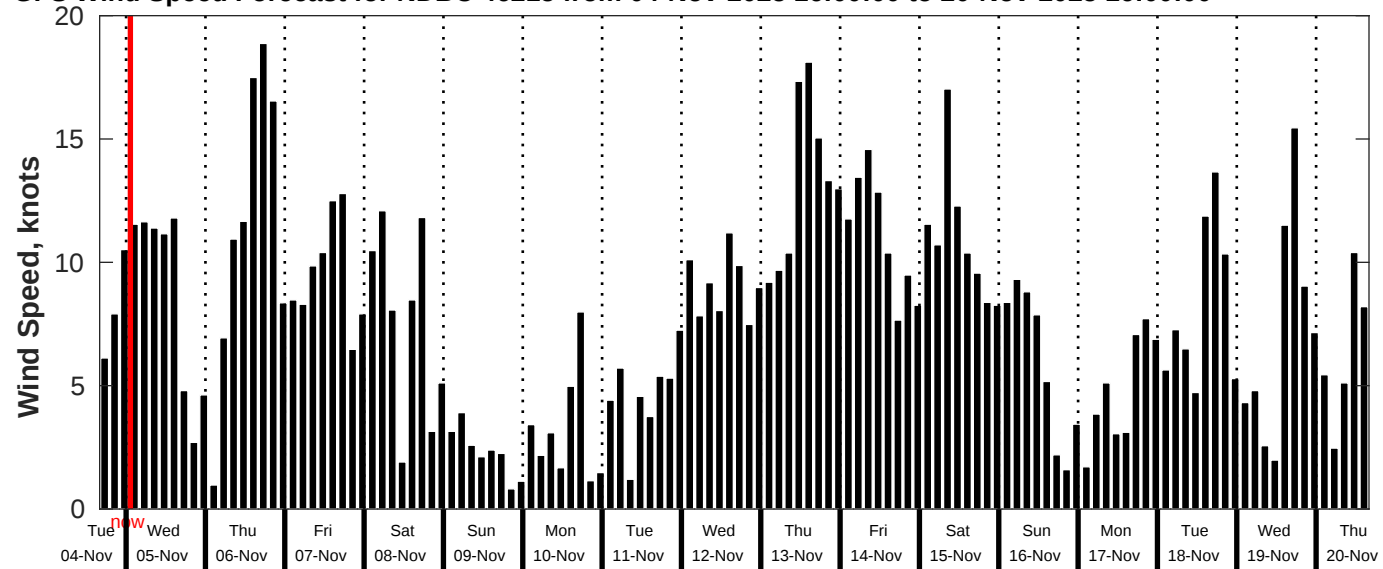
GFS Wind Speed Forecast for NDBC 46215 from 04-Nov-2025 16:00:00 to 20-Nov-2025 16:00:00
