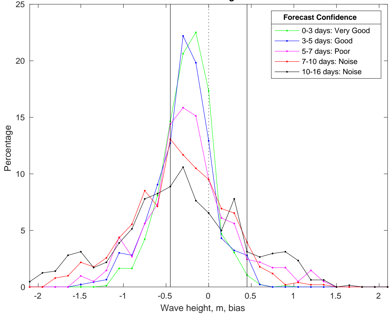
NDBC 46259 vs GFS Waves Bias Histogram: 05-Nov-2025
