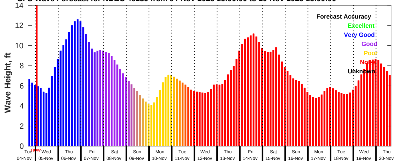
GFS Wave Forecast for NDBC 46259 from 04-Nov-2025 16:00:00 to 20-Nov-2025 16:00:00
