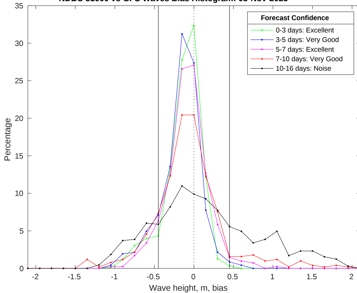
NDBC 51000 vs GFS Waves Bias Histogram: 05-Nov-2025
