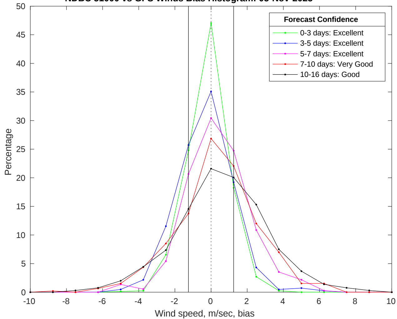
NDBC 51000 vs GFS Winds Bias Histogram: 05-Nov-2025
