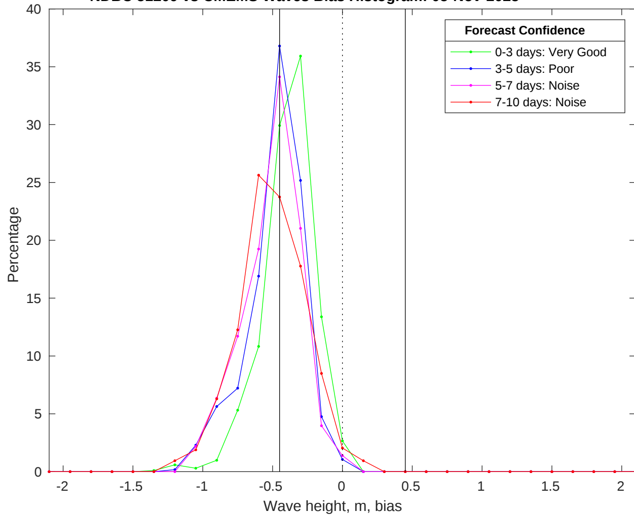
NDBC 51209 vs CMEMS Waves Bias Histogram: 05-Nov-2025
