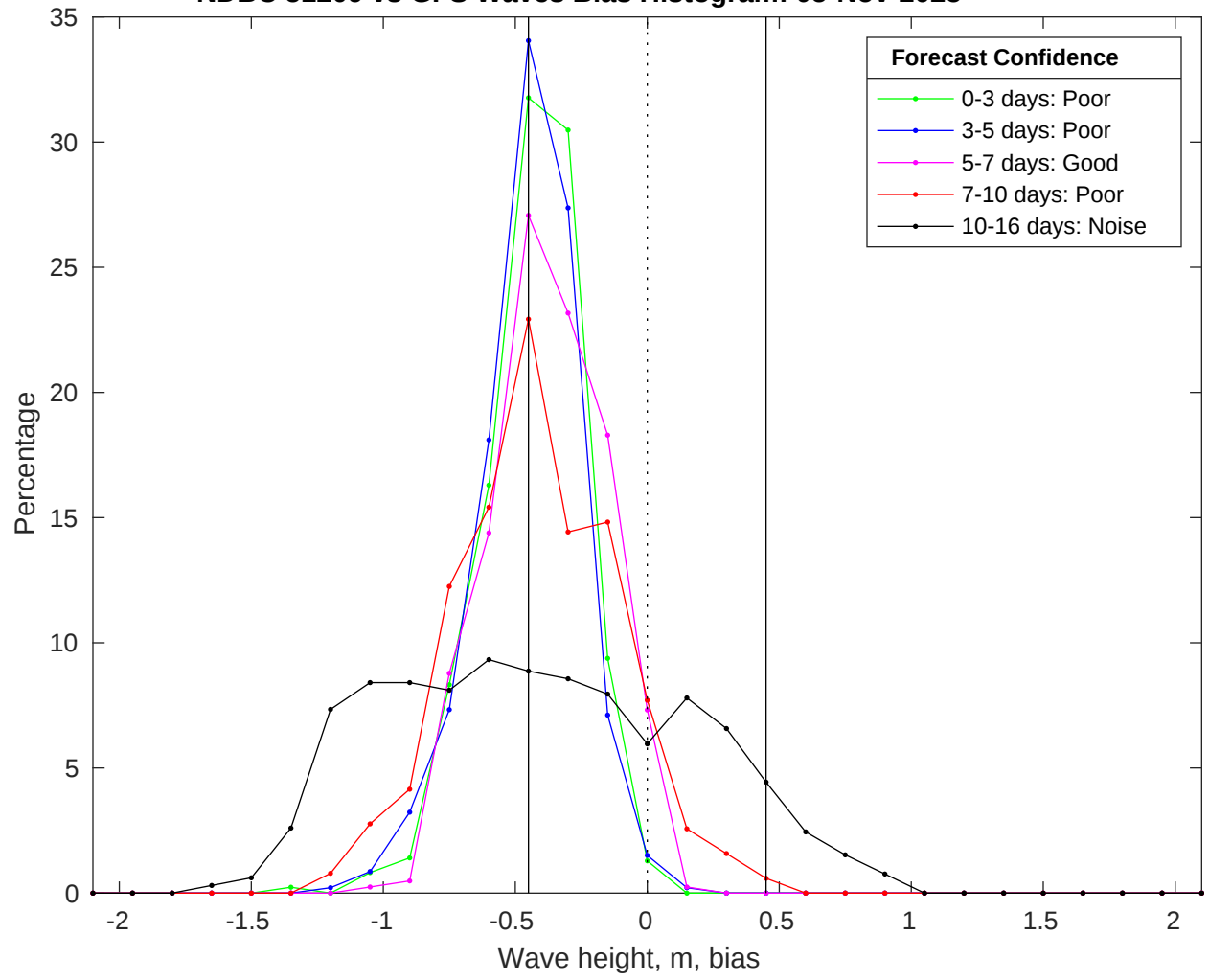
NDBC 51209 vs GFS Waves Bias Histogram: 05-Nov-2025
