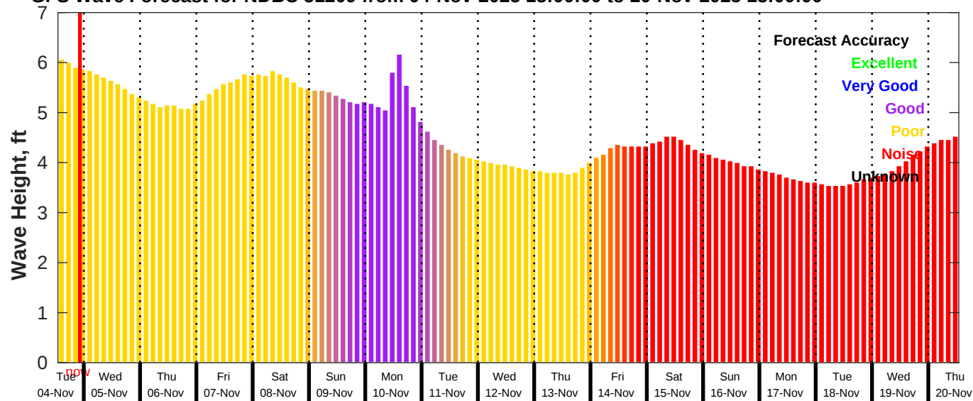
GFS Wave Forecast for NDBC 51209 from 04-Nov-2025 13:00:00 to 20-Nov-2025 13:00:00
