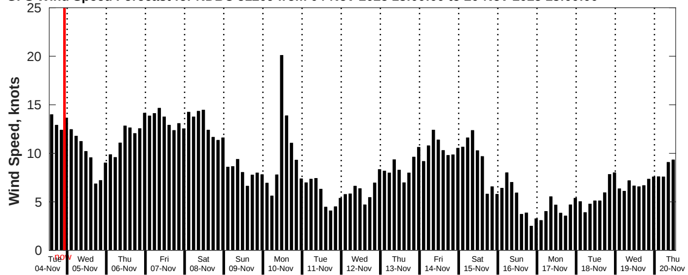
GFS Wind Speed Forecast for NDBC 51209 from 04-Nov-2025 13:00:00 to 20-Nov-2025 13:00:00
