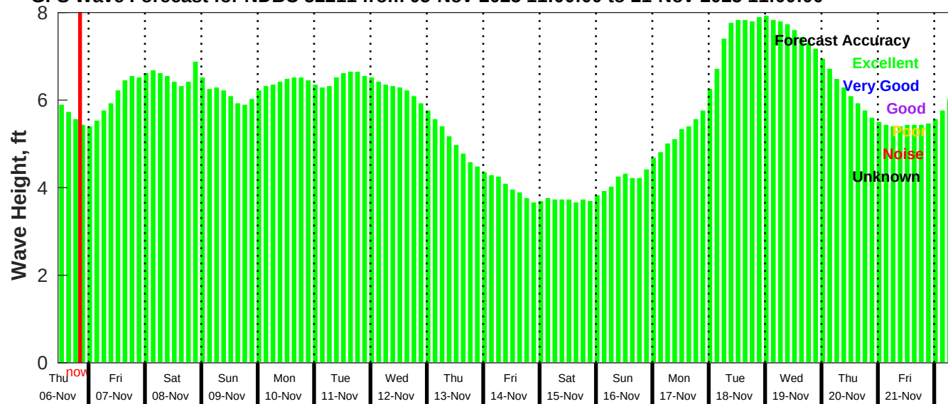
GFS Wave Forecast for NDBC 52211 from 05-Nov-2025 11:00:00 to 21-Nov-2025 11:00:00
