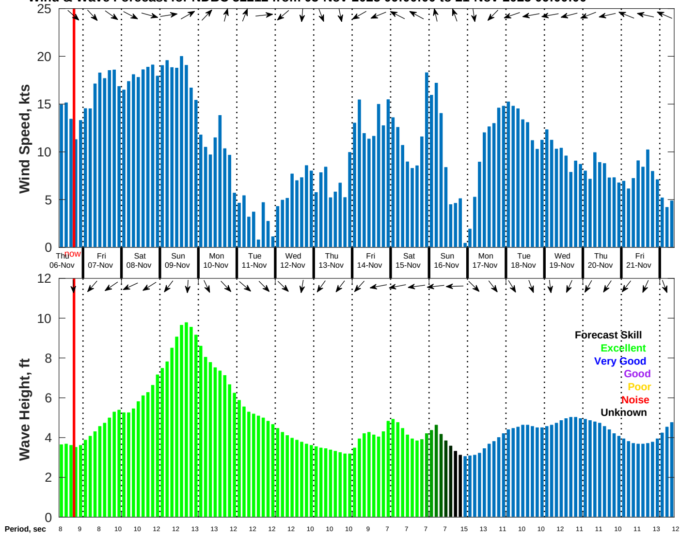
Wind & Wave Forecast for NDBC 52212 from 05-Nov-2025 09:00:00 to 21-Nov-2025 09:00:00
