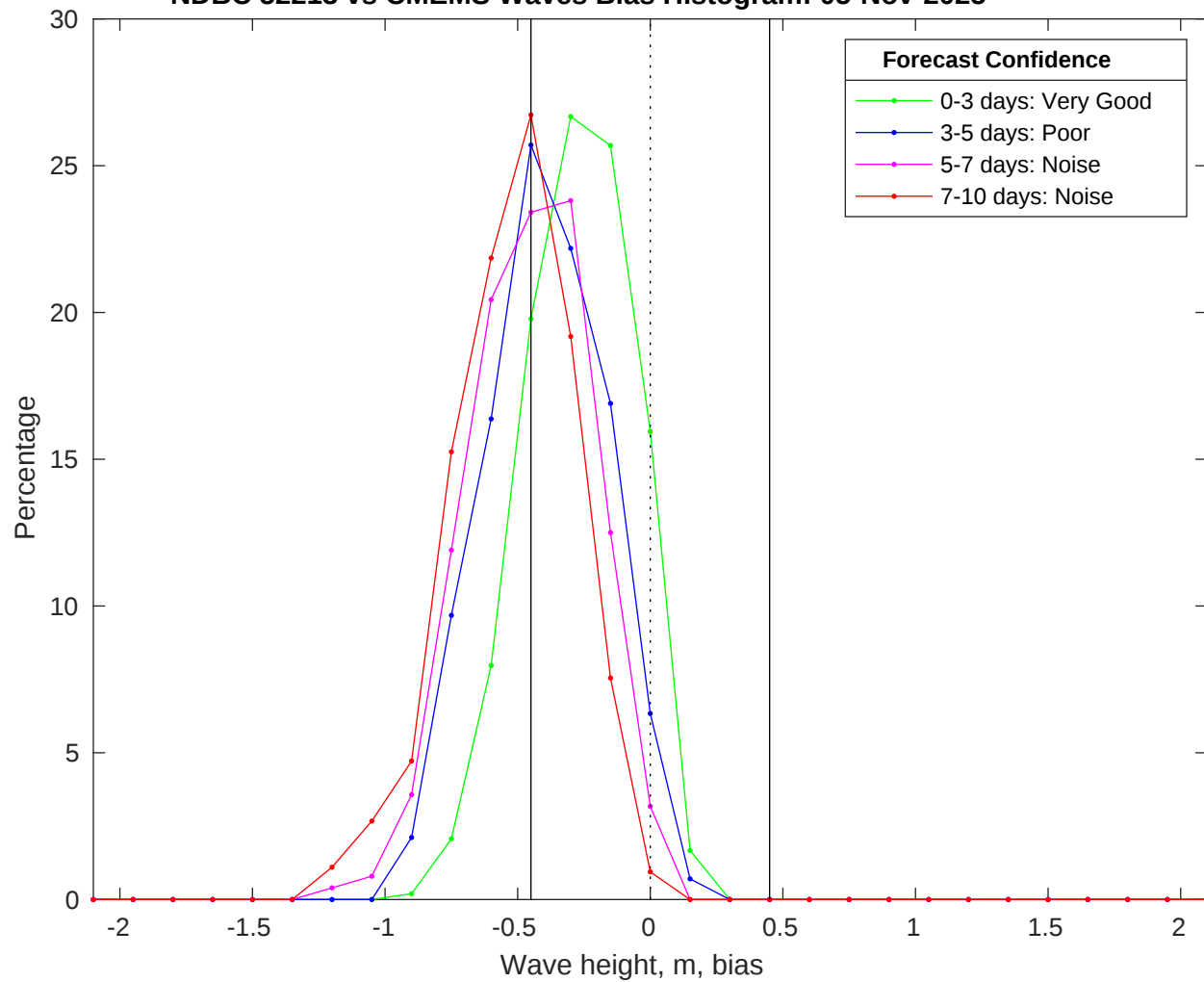
NDBC 52213 vs CMEMS Waves Bias Histogram: 05-Nov-2025
