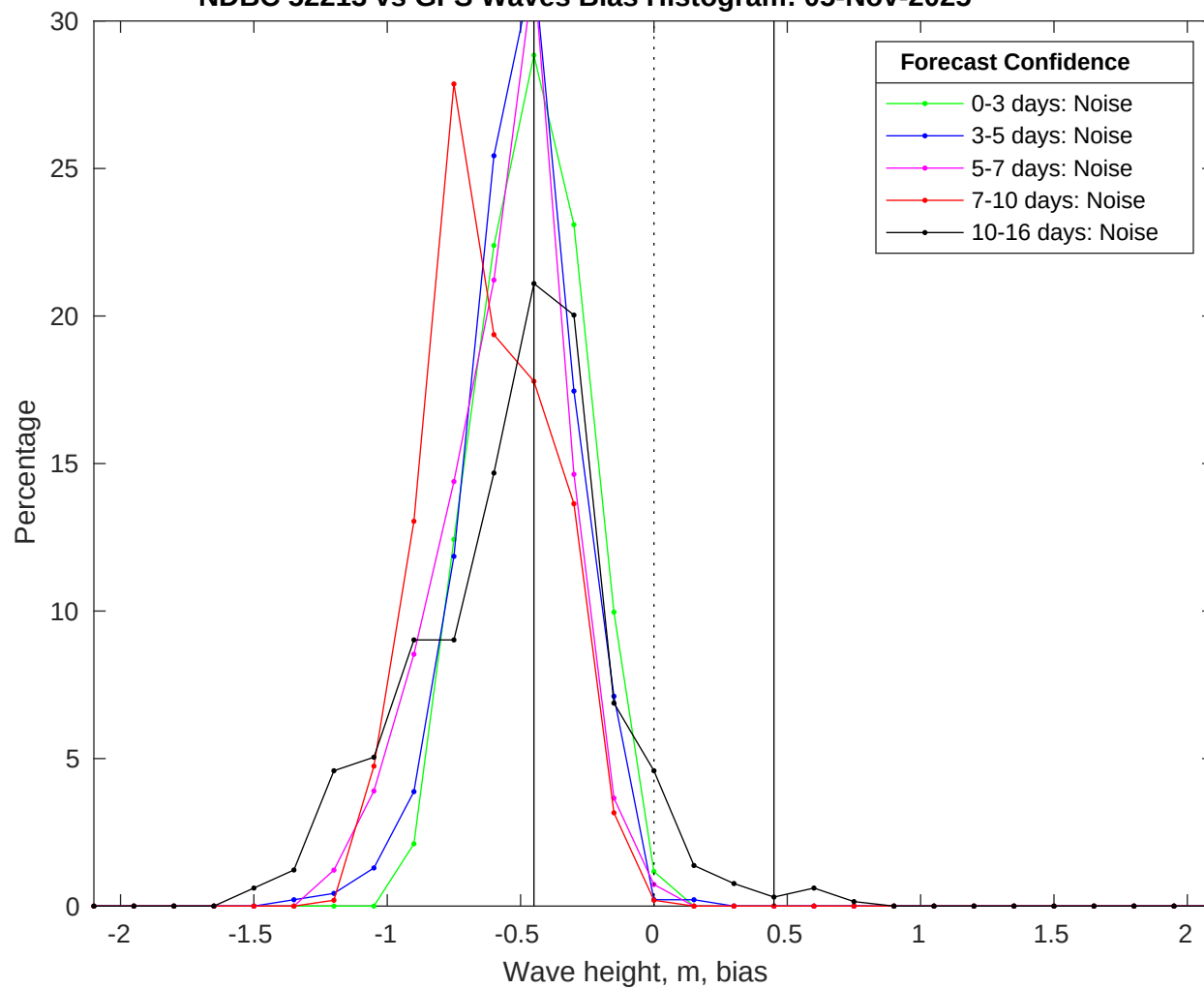
NDBC 52213 vs GFS Waves Bias Histogram: 05-Nov-2025
