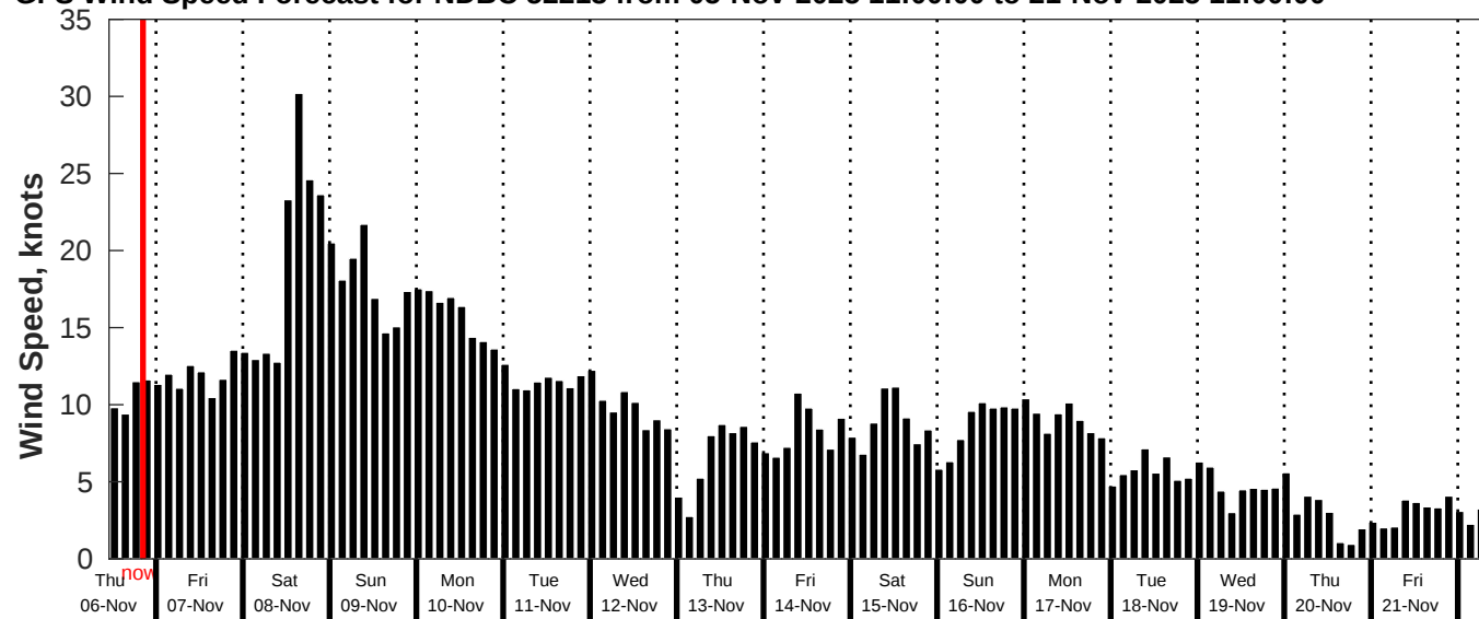
GFS Wind Speed Forecast for NDBC 52213 from 05-Nov-2025 11:00:00 to 21-Nov-2025 11:00:00
