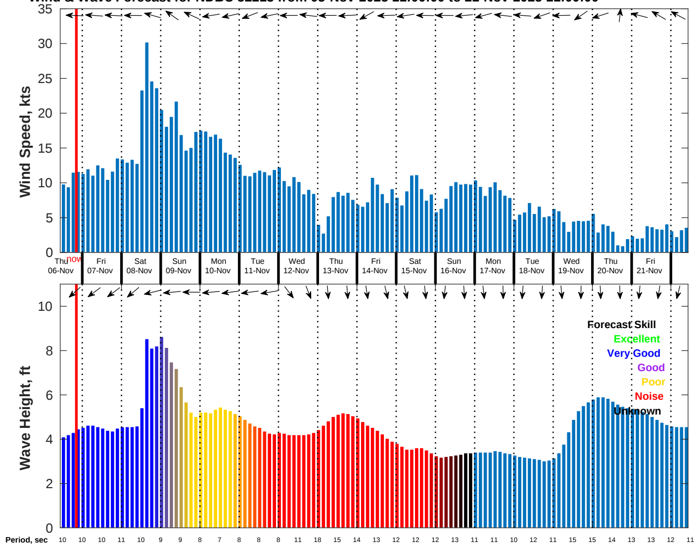
Wind & Wave Forecast for NDBC 52213 from 05-Nov-2025 11:00:00 to 21-Nov-2025 11:00:00
